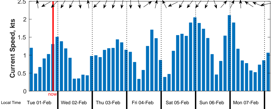
Current Forecast for BP Senegal YT Nearshore from 02-Feb-2022 00:00:00 to 09-Feb-2022 00:00:00
